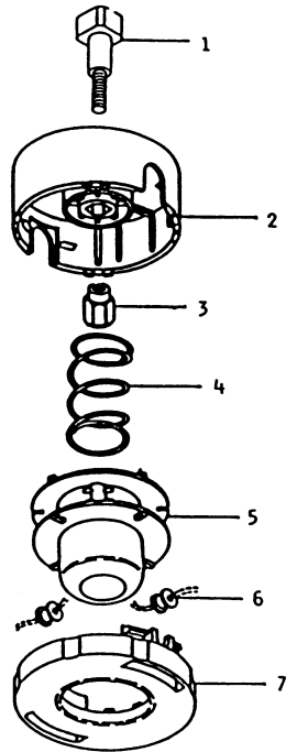
CUTTING HEAD (AUTOMATIC)
